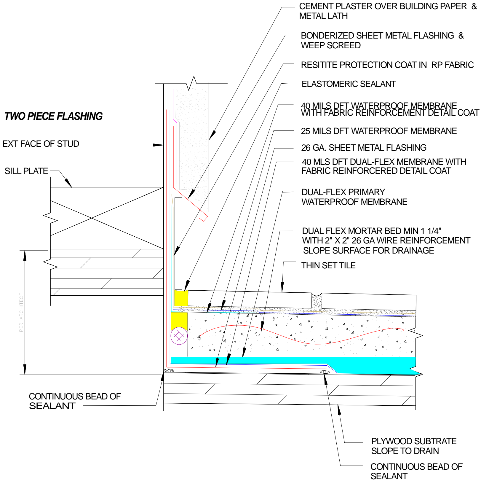
DUAL-FLEX SYSTEM OVER PLYWOOD DECK to WALL
