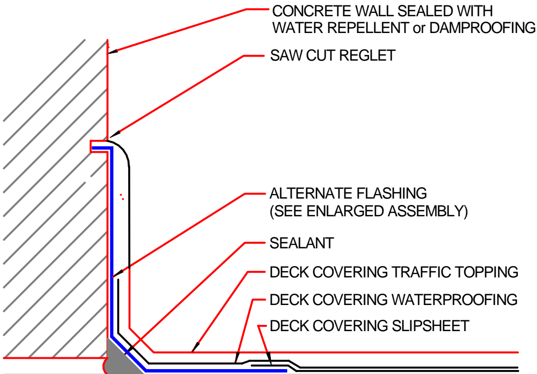
ALTERNATE FLASHING (ENLARGED ASSEMBLY)
