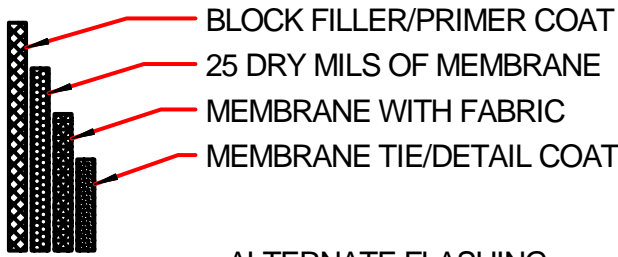
ALTERNATE FLASHING (ENLARGED ASSEMBLY)
