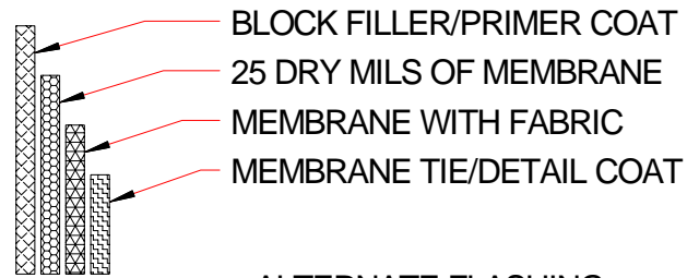
ALTERNATE FLASHING (ENLARGED ASSEMBLY)
